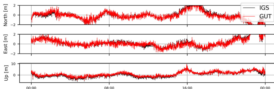
Fig. 13 Time series of topocentric coordinates of the SPTU station located in the area of influence of the storm on November 4, 2021. The red line shows the results obtained using maps generated with the GUT model, while the black line represents the IGS results
