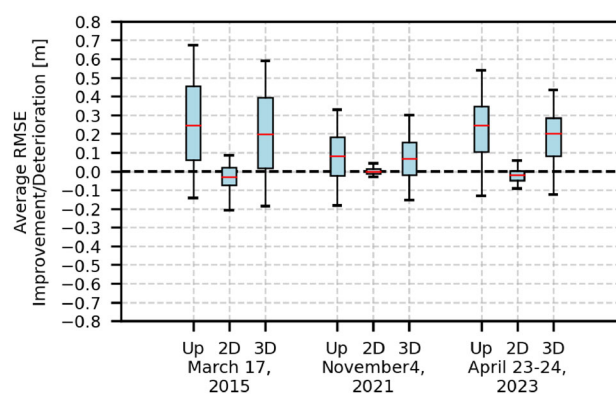
Fig. 12 Comparison of the improvements and deteriorations of the GUT model against the IGS solution for Up, 2D, and 3D positioning error for the studied storm periods: March 17, 2015, November 4, 2021, and April 23–24, 2023. The red line represents the median, the bottom and top of the box indicate the 25th and 75th percentile while the whiskers, lower and upper, indicate the 5th and 95th percentile respectively
