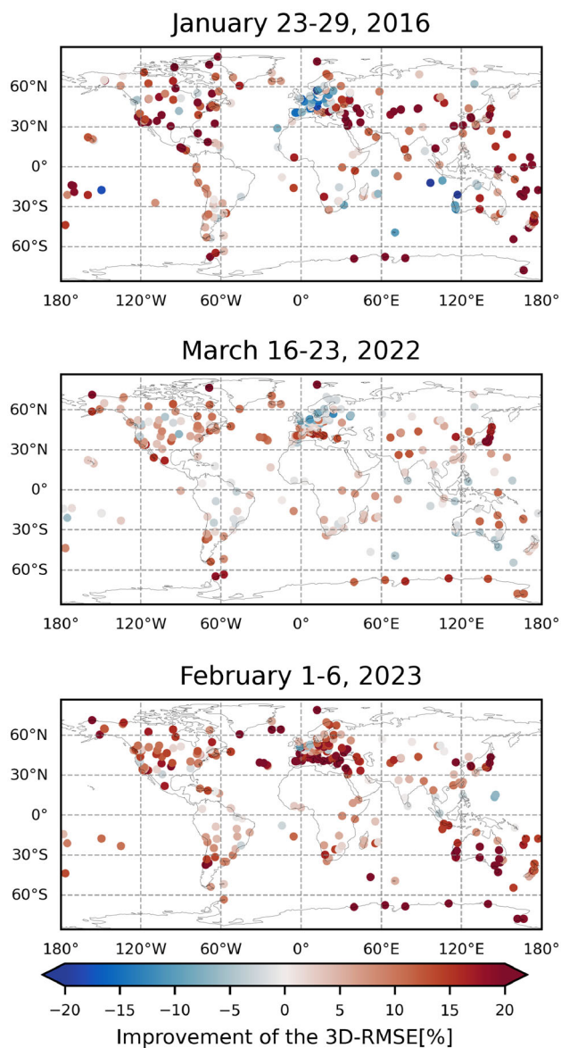
Fig. 7 Spatial distribution of stations showing improvement or deterioration with respect to IGS for the studied quiet periods: January 23–29, 2016, March 16–23, 2022 and February 1–6, 2023
