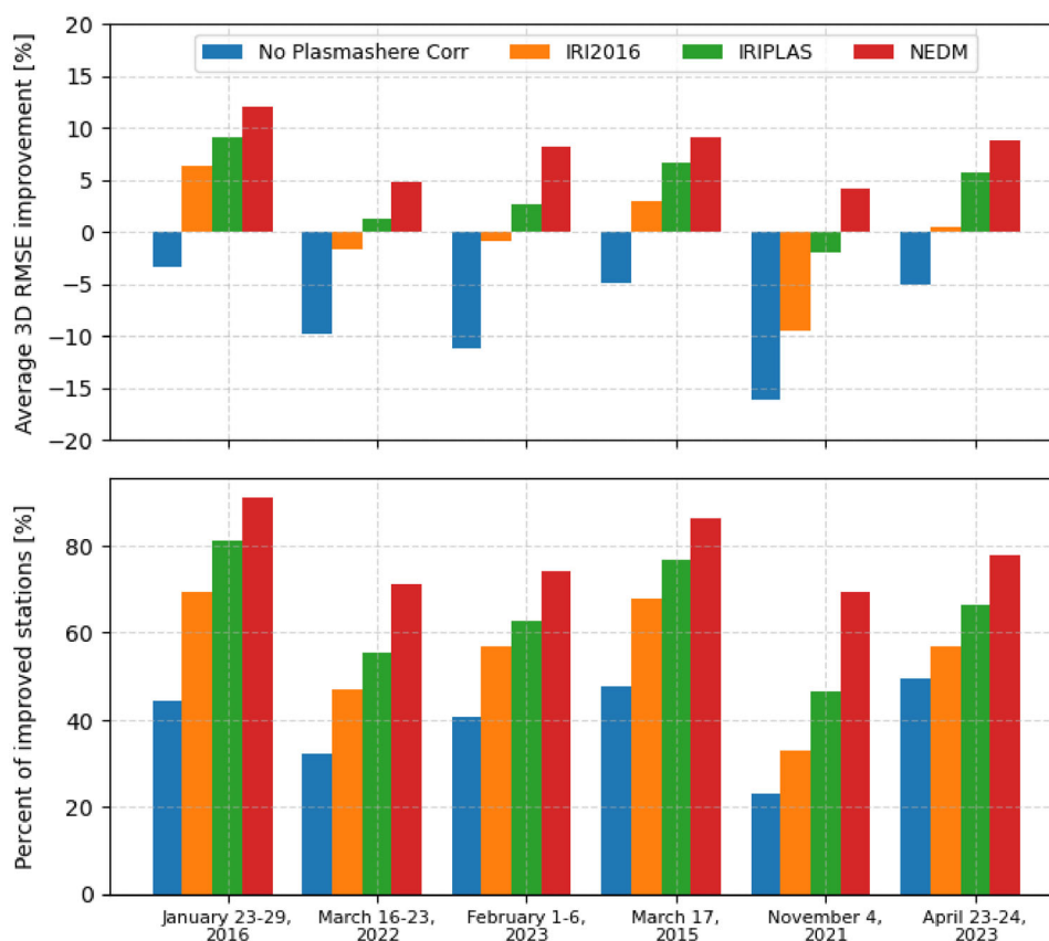
Fig. 14 Comparison of average 3D RMSE improvements for different applied plasmaspheric TEC corrections with respect to solution using final IGS GIM. Blue: no plasmaspheric correction, orange: IRI2016 model, green: IRIPLAS model, red: NEDM
