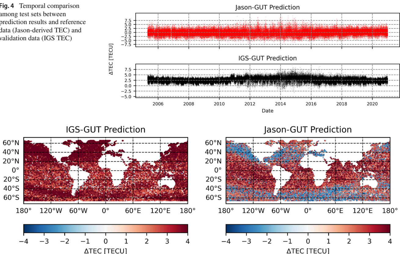
Fig. 5 Spatial comparison among test sets between prediction results and reference data (Jason-derived TEC) and validation data (IGS TEC)
