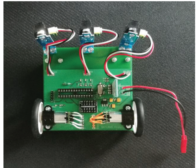
Fig. 10. Top view of the mobile robot
