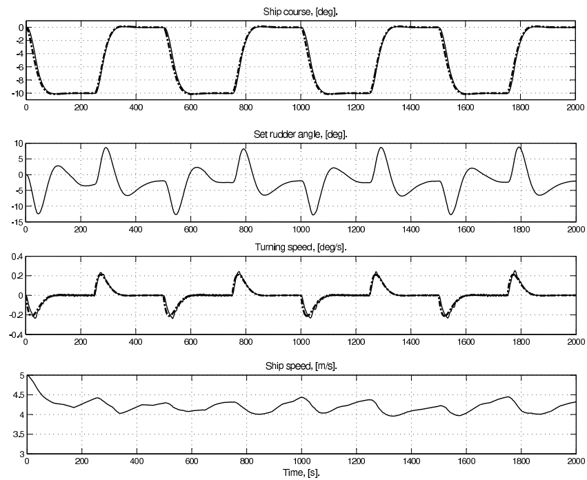
Fig. 7. Time-histories of the ship course, rudder deflection angle, turning speed, ship speed during a programmed change of the set course.
