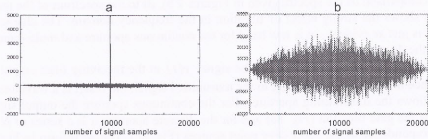
Figure 6. Mutual correlation functions of the signal received along the antenna's main axis ( \vartheta=0^\circ ) and the transmitted signal: (a) S/N = 0 dB and (b) S/N = -25 dB
