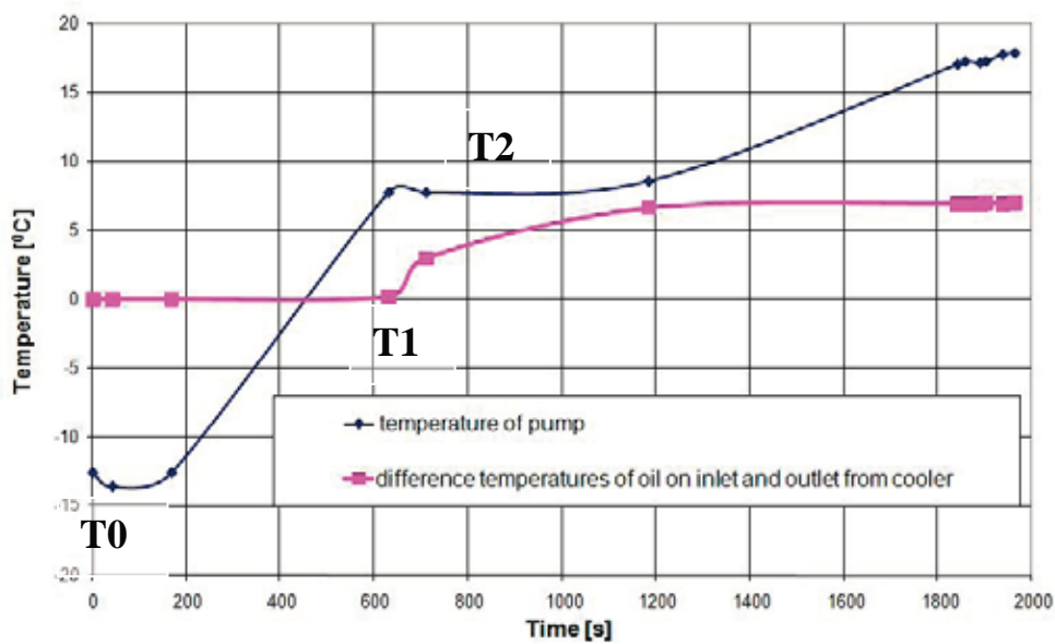
Fig. 5. Pump's housing temperature and difference of temperatures on inlet and outlet from cooler during start-up under following conditions: ambient temperature -12,6\text{ }^{\circ}\text{C} , flow rate in the closed loop circuit 156\text{ dm}^3/\text{min} , pump's shaft rotation speed 1570\text{ rpm}
