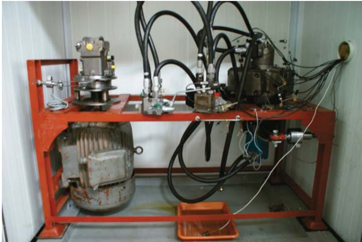
Fig. 10. Laboratory stand for testing hydraulic component [12-17] and system placed in the low temperature chamber
