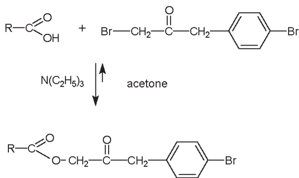
Figure 1. Scheme of the free fatty acid derivatization reaction.
