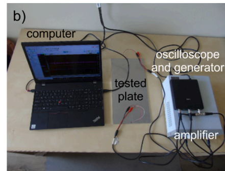
Fig. 4. Experimental setup: a) configuration of the transducers and b) used instrumentation.
