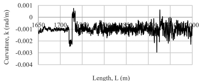
Fig. 9. Curvature waveform illustrating satellite signal quality deterioration
