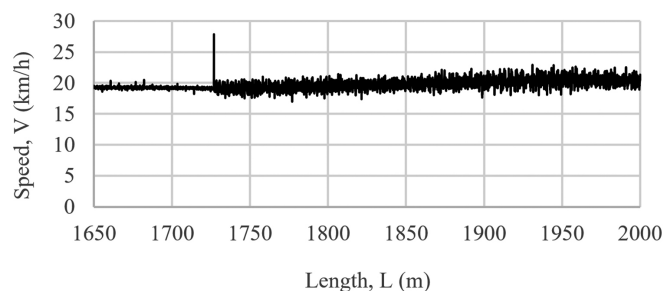
Fig. 10. Speed of measuring trolley in the region of satellite signal quality deterioration
