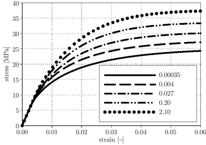
Figure 2. Uniaxial tension tests for various strain rates [ \text{s}^{-1} ]
