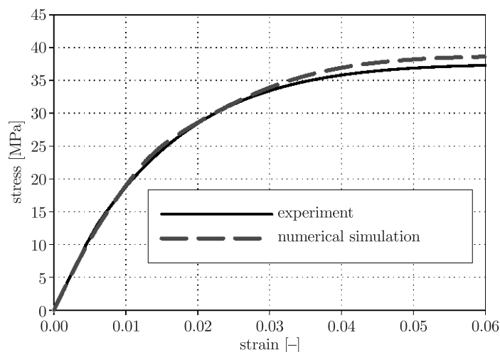
Figure 10. Results of a B-P simulation of a uniaxial tension test for \dot{\varepsilon} = 2.10\text{s}^{-1}
