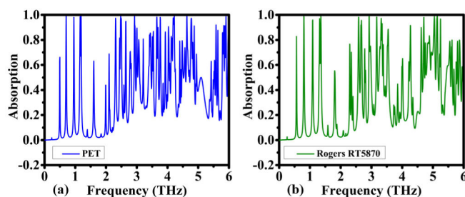
Fig. 5. Absorption spectra for the proposed design under different substrates. (a) PET. (b) Rogers RT 5870.
