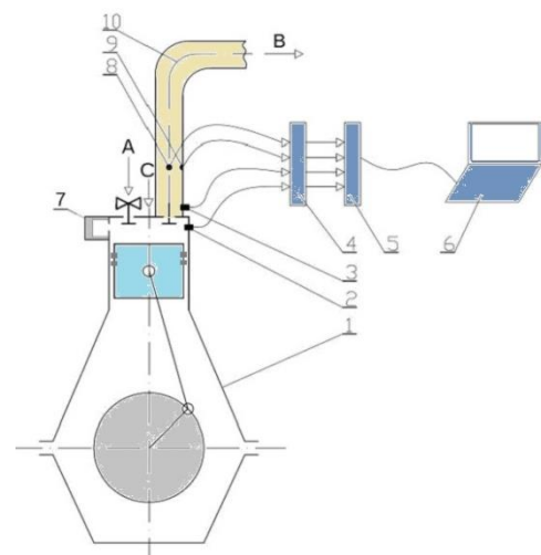
Fig. 12. Schematic of the laboratory bench with the mounting locations of the measurement sensors marked: 1 – test engine, 2 – TDC piston position and crankshaft rotational speed sensor, 3 – exhaust valve opening sensor, 4 – A/C converter, 5 – recorder, 6 – analysis software, 7 – structural element enlarging the volume of the combustion chamber, 8 – exhaust gas pressure sensor, 9 – thermocouple for rapidly variable measurements, 10 – exhaust gas channel, A – intake air, B – exhaust gas, C – supply fuel
