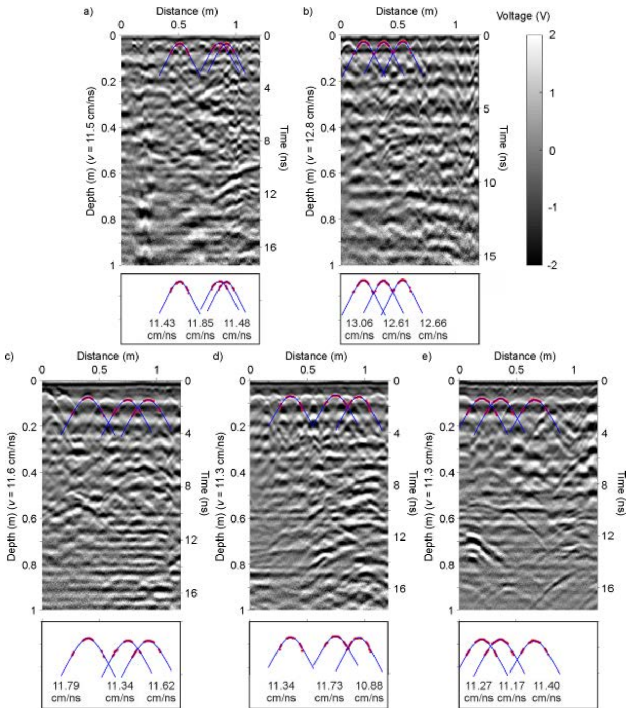
Figure 11. Longitudinal GPR maps with estimated velocity values from measurements of strengthened masonry pillars: a) pillar S.1 b) pillar S.2 c) pillar S.3 d) pillar S.4 e) pillar S.5
