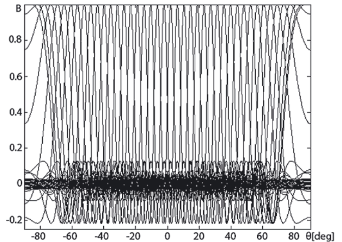
Fig. 8. Equally spaced sonar beams
