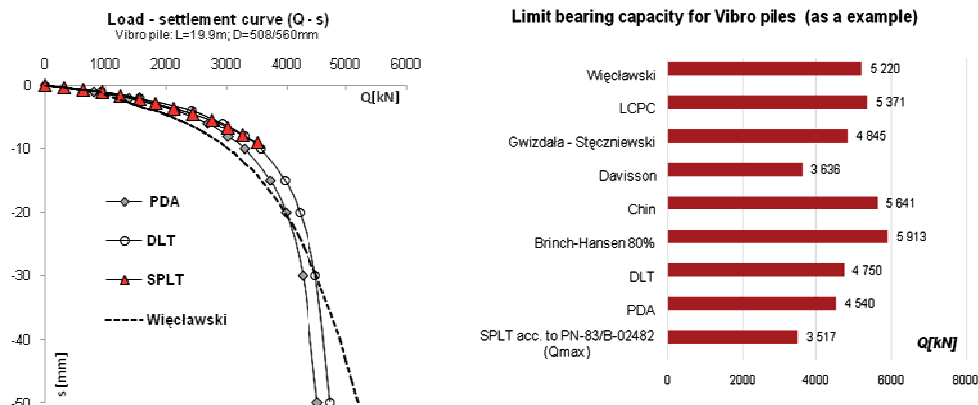
FIGURE 9. Summary of the results of the limit load capacity obtained on the basis of analytical methods and field tests for Vibro pile: L = 19.9 m, D = 508/560 mm (Gwizdała, 2013)
