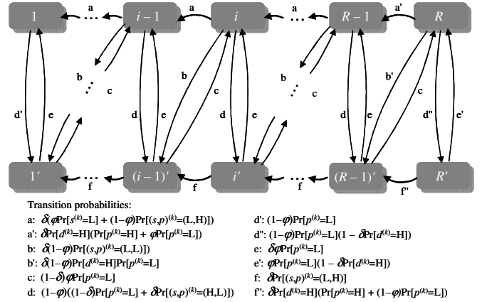
Fig. 4. Two-dimensional Markov chain for iFVIP.
