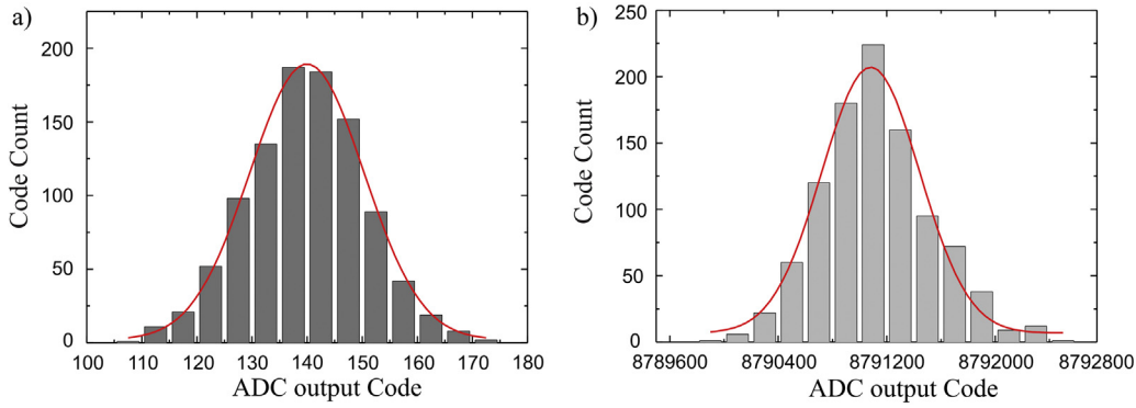
Fig. 1. Random noise histogram for 1000 total number of codes with grounded input (a) and for a half-scale input from photo detection unit (b).
