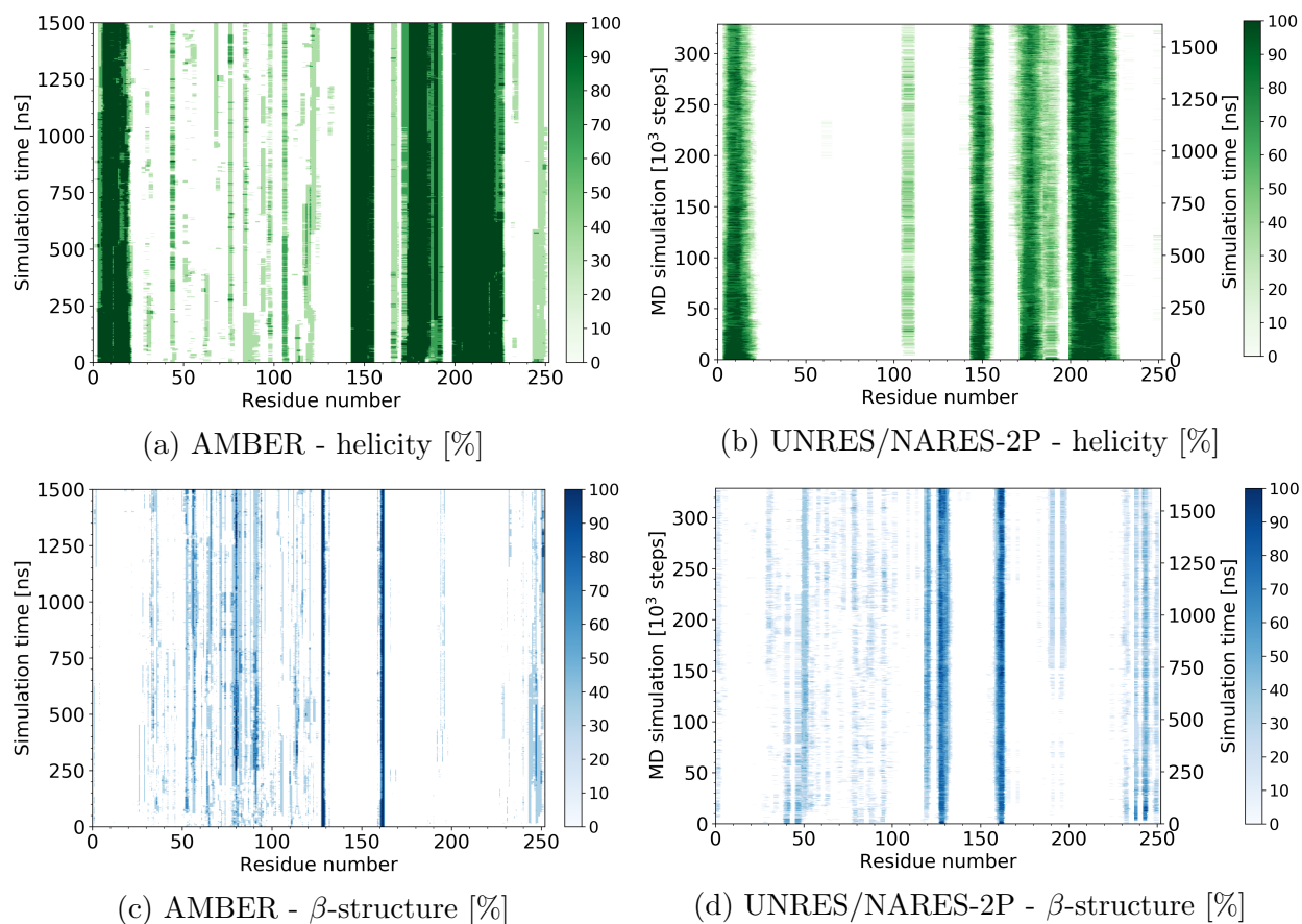
Figure 1: Time evolution of secondary structure as measured for the 129M-178D prion-RNA complex secondary structure in all-atom (AMBER) simulations (a and c), and in coarse-grained (UNRES) (b and d) simulations. The helical fragments are marked in green colors (a and b), and the \beta -strands in blue (c and d). The colors intensity corresponds to the frequency of occurrence of the secondary structure. All trajectories start with RNA bound to the binding site 3 of the wild type 129M-178D prion.
