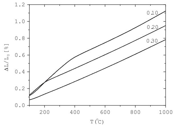
Fig. 7. Relative length change of the \text{LaNb}_{1-x}\text{Sb}_x\text{O}_4 samples as a function of temperature.
