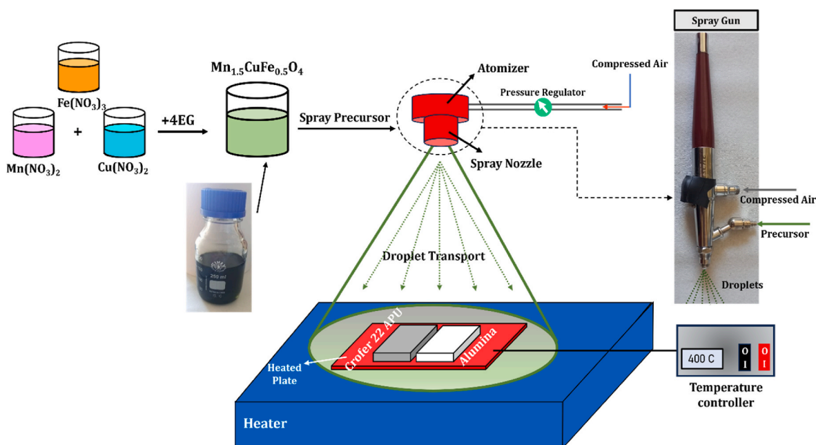
Fig. 1. Schematic illustration of spray pyrolysis method used for preparation of \text{Mn}_{1.5}\text{CuFe}_{0.5}\text{O}_4 spinel oxide coatings in this research.
