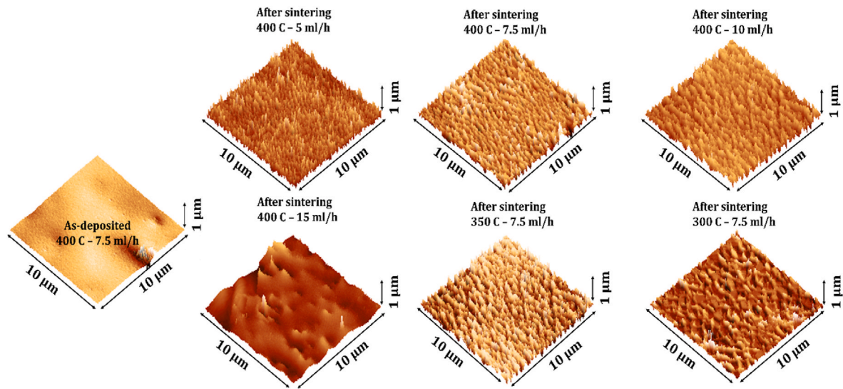
Fig. 9. AFM images in 10 \times 10 \mu\text{m}^2 of surface area of the deposited \text{Mn}_{1.5}\text{CuFe}_{0.5}\text{O}_4 spinel oxide coatings at temperature of 300, 350 and 400 °C with spraying speed of 5, 7.5, 10 and 15 ml/h, before and after sintering at 800 °C for 3 h.
