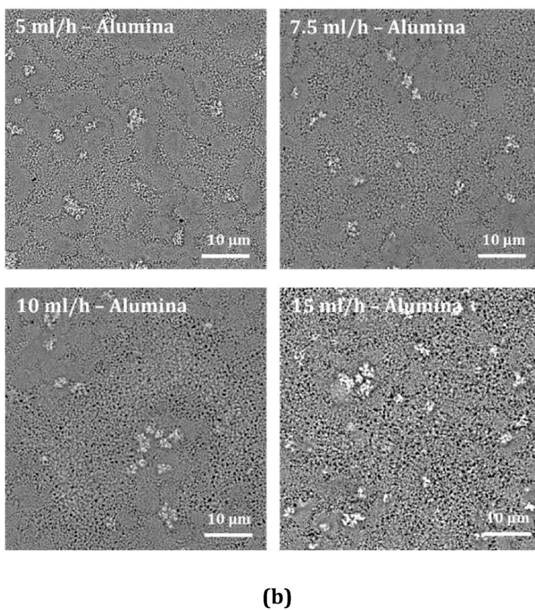
Fig. 5. The top-view SEM images of the microstructure of deposited \text{Mn}_{1.5}\text{CuFe}_{0.5}\text{O}_4 spinel oxide coatings on: (a) Crofer 22 APU and (b) alumina substrates with different spraying speeds at deposition temperature of 400 °C and 100 ml of precursor.
