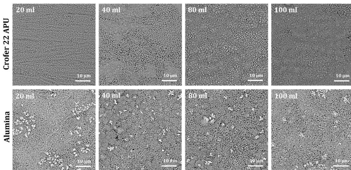
Fig. 6. Top-view SEM images showing microstructure of the deposited \text{Mn}_{1.5}\text{CuFe}_{0.5}\text{O}_4 spinel oxide coatings with different volume of the precursors on Crofer 22 APU and alumina.
