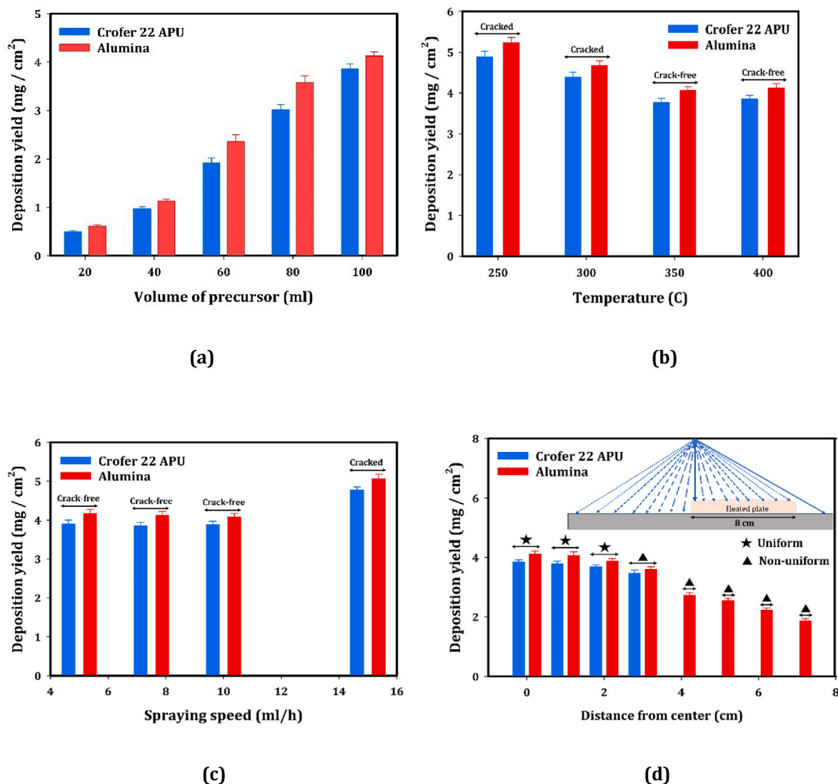
Fig. 2. Deposition yield of prepared spinel oxide coatings by spray pyrolysis method as a function of (a) volume of precursor, (b) deposition temperature, (c) spraying speed, (d) distance of center.
