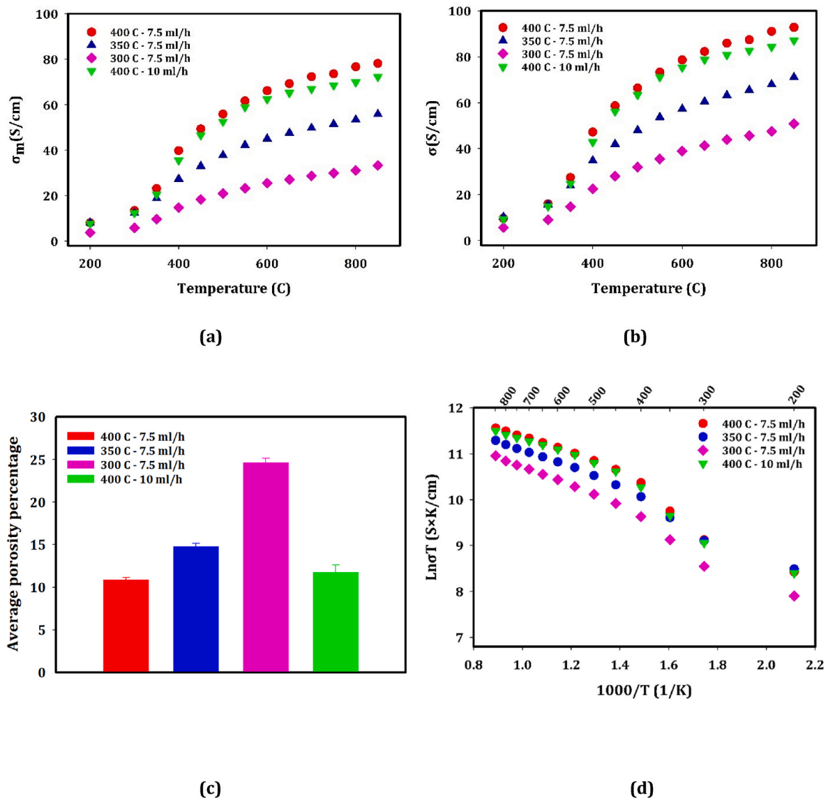
Fig. 11. (a) Measured electrical conductivity of the deposited spinel oxide coatings at the different temperatures and spraying speeds, (b) electrical conductivity of the deposited spinel oxide coatings at the different temperatures and spraying speeds modified with the average porosity percentage, (c) the measured average porosity percentage of the deposited spinel oxide coatings at the different temperatures and spraying speeds, and (d) Arrhenius diagram presenting the correlation between electrical conductivity and applied temperature during Van Der Pauw measurement for the deposited spinel oxide coatings.
