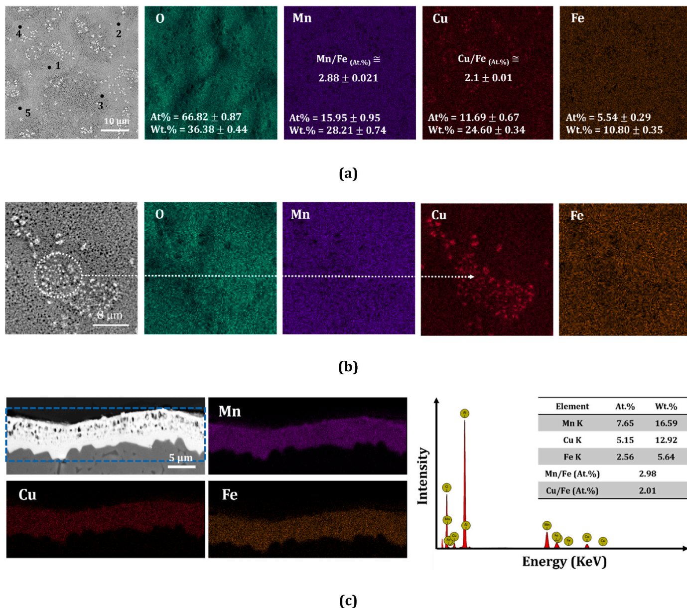
Fig. 4. (a) Elemental analyses showing the elemental distribution across the surface of the deposited coating and the chemical composition at designated points; (b) high-magnification mapping results showing Cu precipitates on the surface; and (c) elemental analyses showing the elemental distribution and chemical composition across the cross section of the deposited coating (larger area). The coatings were produced at 300 °C (c) and 400 °C (a and b) with a spraying speed of 7.5 ml/h using 100 ml of precursor on an alumina substrate.
