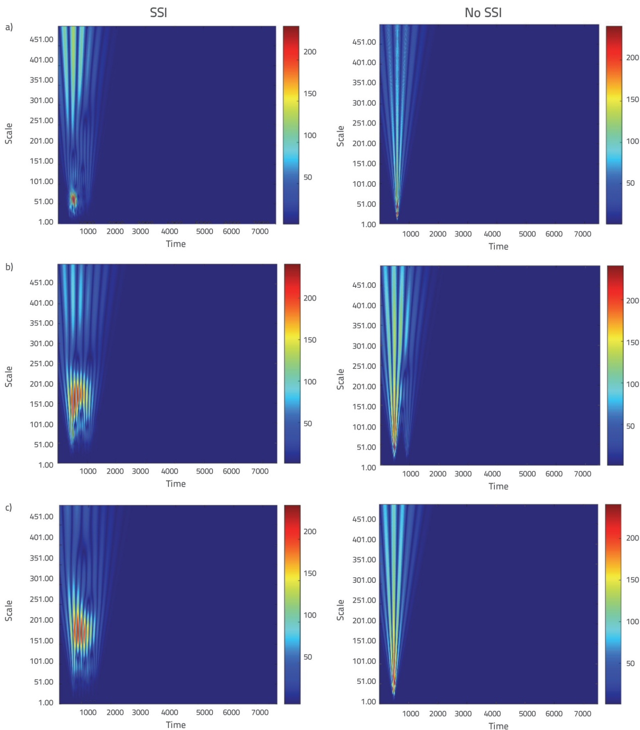
Figure 6. Wavelet scalogram of impact forces in case 3 under the Kobe earthquake: a) 15/5 storeys; b) 15/10 storeys; c) 15/15 storeys
