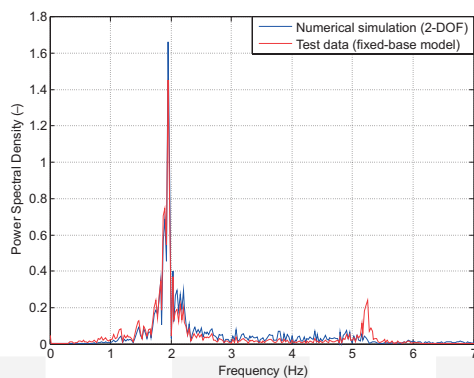
Fig. 12. Comparison between the FFT functions for the fixed-base model under the 1940 El Centro earthquake
