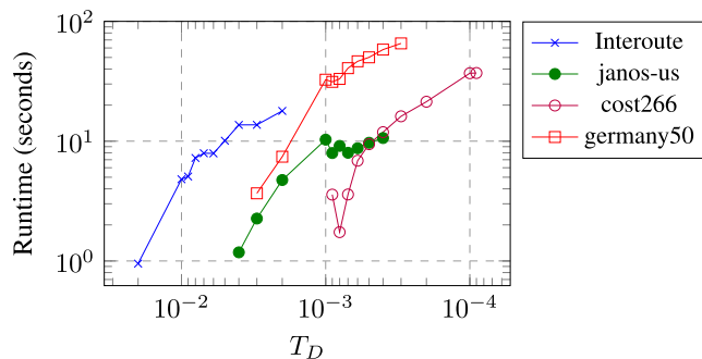
FIGURE 12. Comparison of the computation time values of the DPH upgrade method for different networks and probability thresholds ( T_D ). For each network the upgrade is computed for 10 T_D values.
