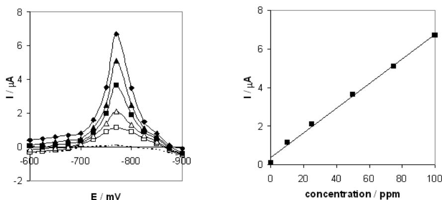
Fig. 6. SWV voltamograms obtained for the sensor exposed to the gaseous mixtures dry air/benzaldehyde. Internal electrolyte 1-hexyl, 3-methylimidazolium chloride. Dry air-dashed line. ( \square ) – 10 ppm v/v, ( \triangle ) – 25 ppm v/v, ( \blacksquare ) – 50 ppm v/v ( \blacktriangle ) – 75 ppm v/v, ( \blacklozenge ) – 100 ppm v/v of benzaldehyde. Right plot – calibration curve of the sensor for measurement of benzaldehyde in air, obtained based on the SWV voltamograms.
