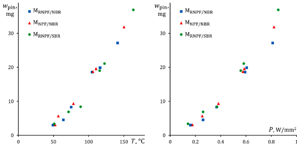
Fig. 14. Dependencies of the pin sample wear w_{pin} on the temperature T and specific power P .
