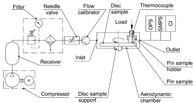
Fig. 2. Experimental set-up.
