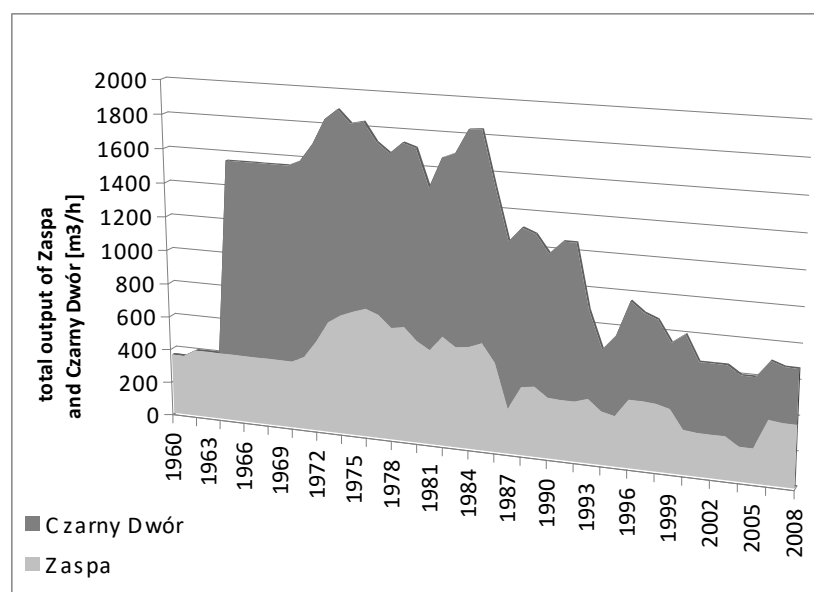
Fig. 6 Total output from the Quaternary aquifer on the intakes Zaspa and Czarny Dwór (cumulative graph - the upper line shows the sum of groundwater exploitation)
