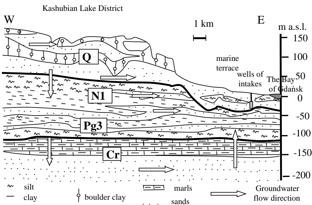
Fig. 3 Schematic hydrogeological cross-section from the Kashubian Lake District to the marine terrace and the Bay of Gdańsk.
