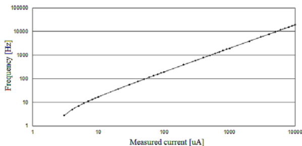
Fig. 5. Relationship between charge counts and current for analog charge integration method
