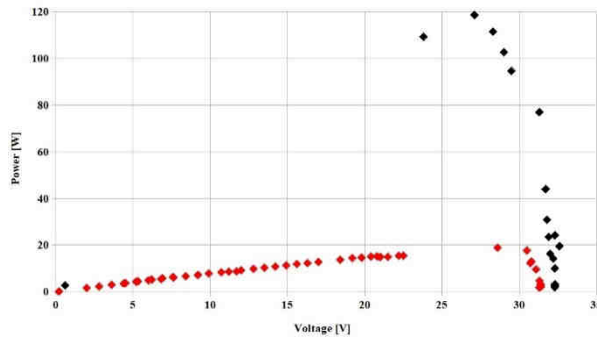
Fig. 12. Power-voltage characteristic at 632 \text{ W/m}^2 irradiance without shade (black colour) and with natural shade (red colour)
