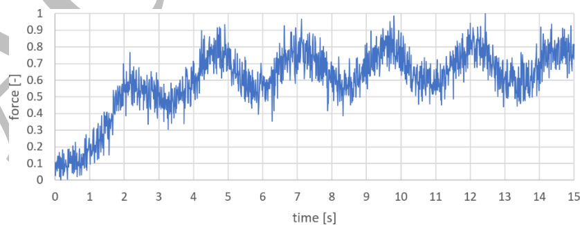
Fig. 2. Chosen normalised internal force values in time for model tuned to the data from [30].
