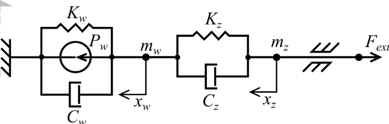
Fig. 1. Considered rheological model, where K_w , K_z – stiffness of active and passive tissues, C_w , C_z – damping of active and passive tissues respectively, m_w , m_z – mass of active and passive tissues, x_w – displacement of active tissue, x_z – displacement of the system, P_w – force generated by active tissue, F_{ext} – external force.
