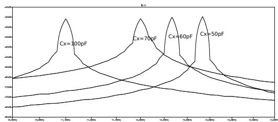
Fig. 11. Parametric analysis of the signal frequency versus sensor capacitance
