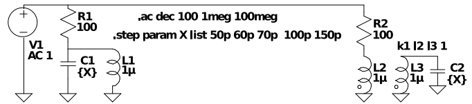
Fig. 6. Test schematic used for the simulation
