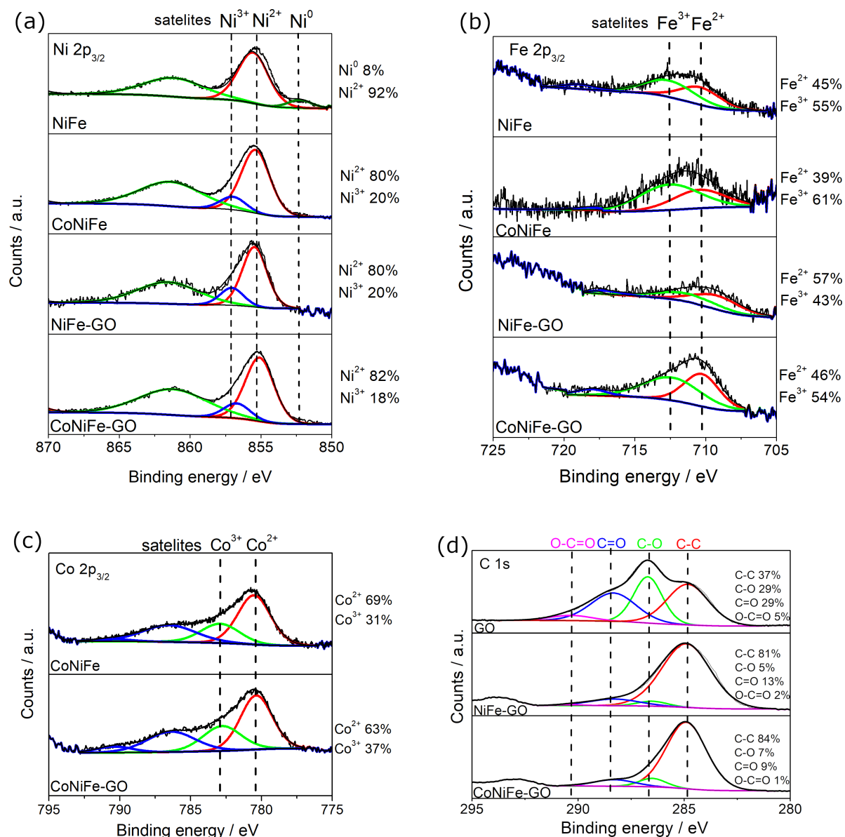
Figure 4: XPS high-resolution spectra of Ni 2p (a), Fe 2p (b), Co 2p (c), and C 1s (d) levels of the catalysts with the determined surface concentration of the elements (error \leq 5\% ).
