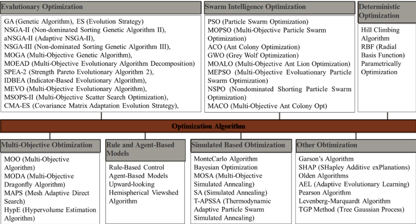
Fig. 7. Categorization of optimization algorithms in studies.
