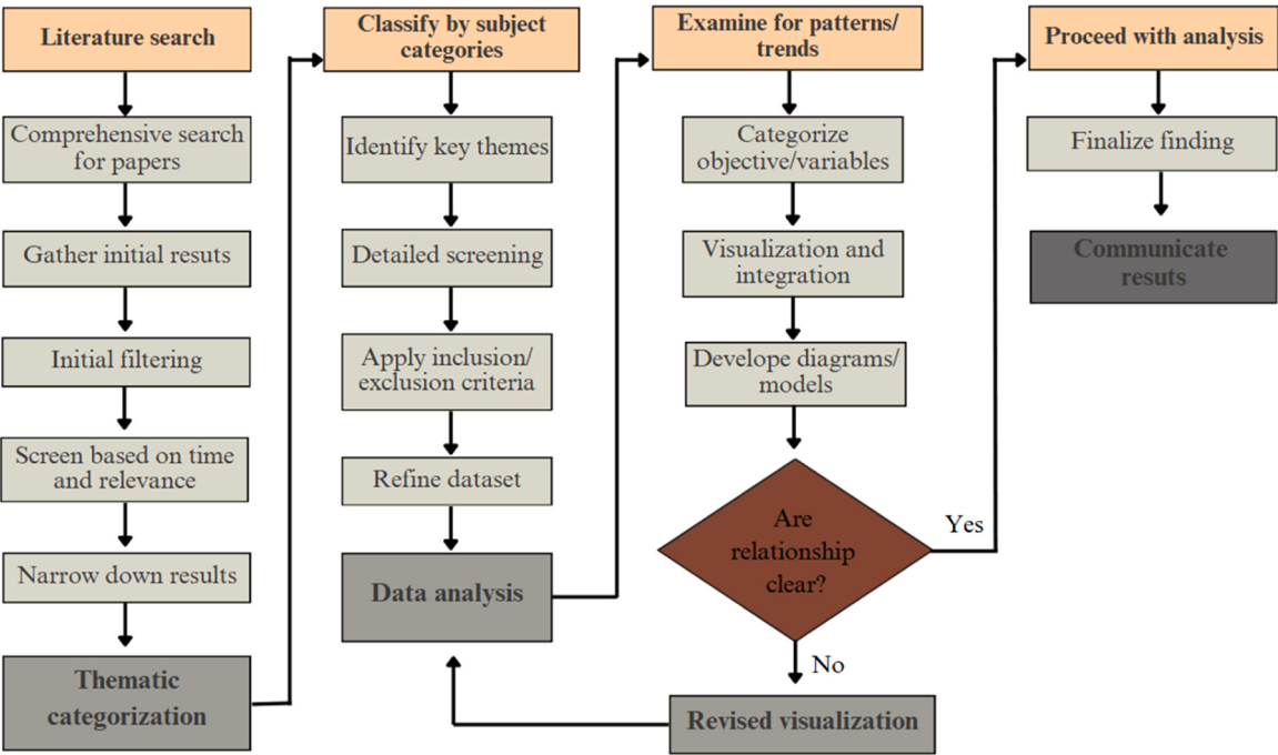
Fig. 2. Methodology flowchart.
