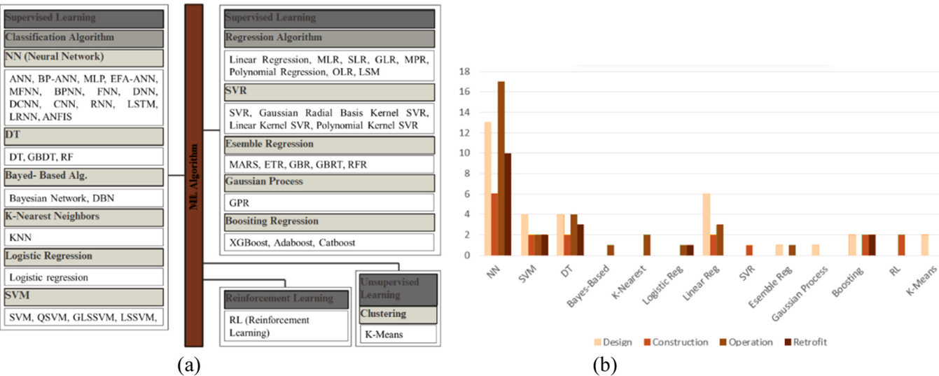
Fig. 5. (a) Classification of ML algorithms used in energy studies in buildings, (b) Number of ML algorithm classes used in LC processes.
