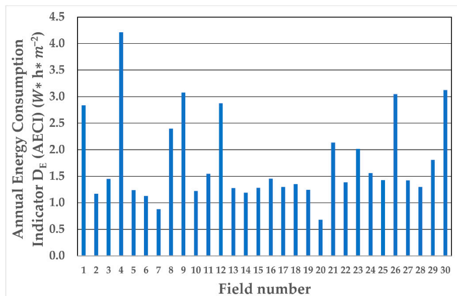
Figure 15. D_E (AECI) Annual Energy Consumption Indicator ( W * h * m^{-2} ) in calculation fields.
