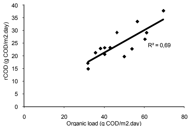
Fig. 1. COD mass loading vs. removal rate
