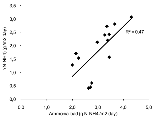
Fig. 3. N-NH 4 mass loading vs. N-NH 4 removal rate
