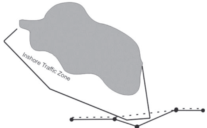
Fig. 8. Fixing violations of inshore zone - shifting the first node of a segment
