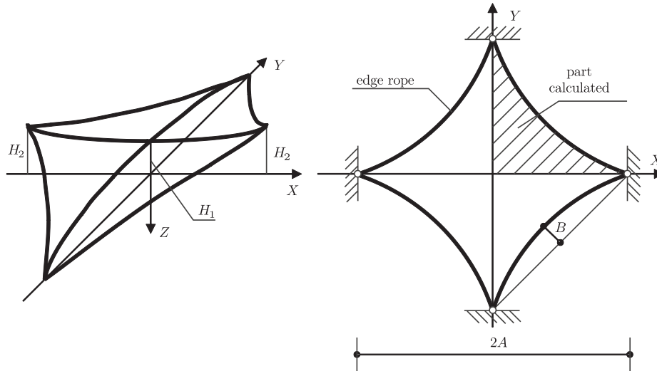
Figure 4. Roof geometry
