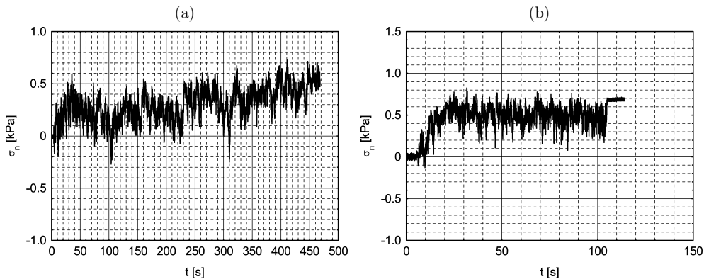
Figure 2. Measured horizontal wall pressure, \sigma_n , at h = 1.0 m for controlled outlet velocity: (a) v = 0.7 mm/s; (b) v = 5 mm/s (cylindrical silo, loose sand, d_{50} = 0.8 mm, smooth walls)
