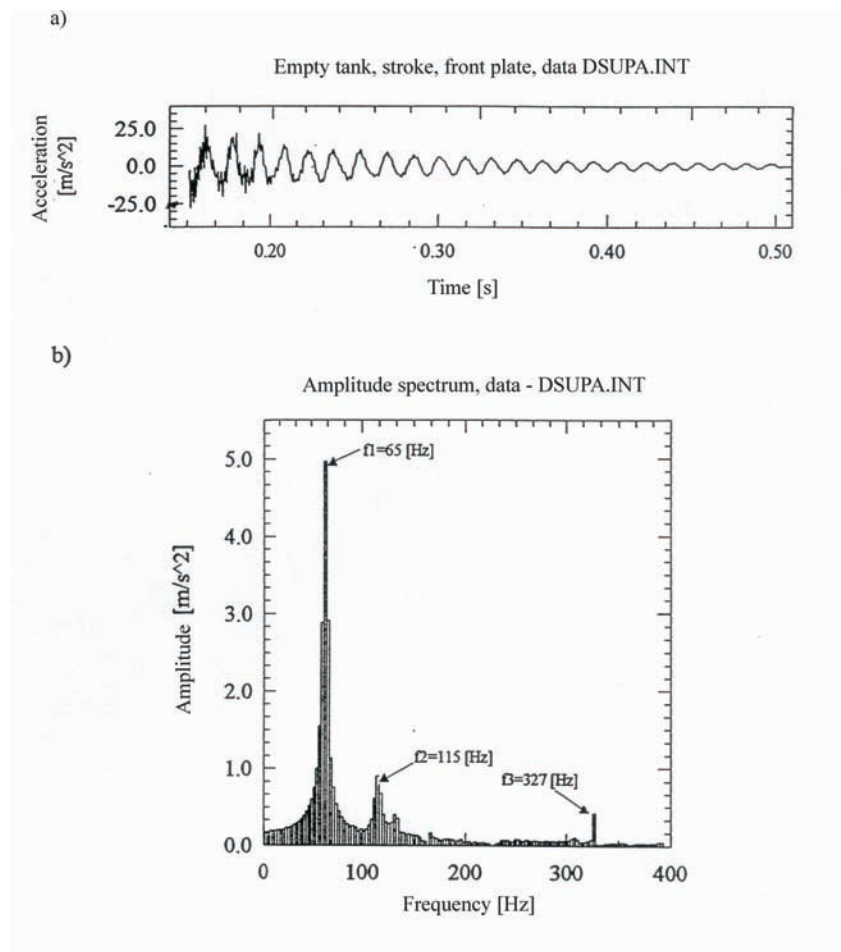
Fig. 7. Records of plate centre acceleration (a) and amplitude spectrum of its vibrations (b)
