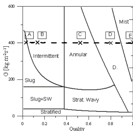
Figure 3. Flow pattern map
