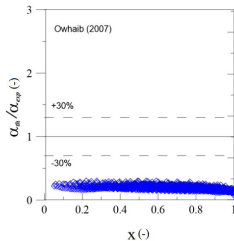
Figure 35. Comparison of the test results using the Owhaib (2007) correlation as a function of vapour quality.
