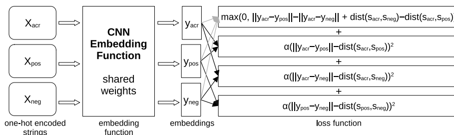
Fig. 3. Triplet Loss Network architecture.
