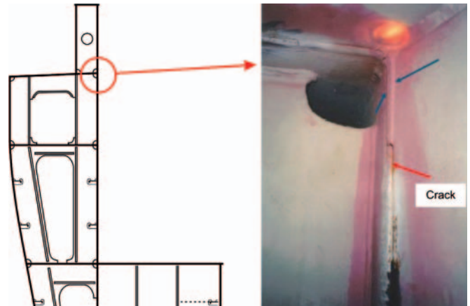
Fig. 3. Example of fatigue crack in welded joint of ship structure detail of a containership [3]
