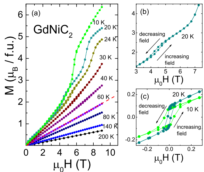
FIG. 2. (a) Magnetisation of \text{GdNiC}_2 measured at various temperatures as a function of H . (b) and (c) show the expanded views of hysteresis observed at high and low fields, respectively.
