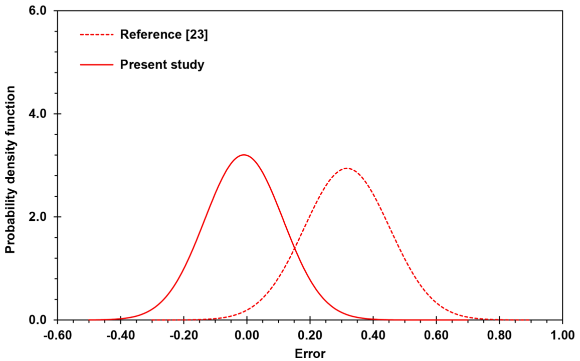
Fig. 9. Probability density functions defined from the predictive error for both fatigue life prediction models considered in this study.
