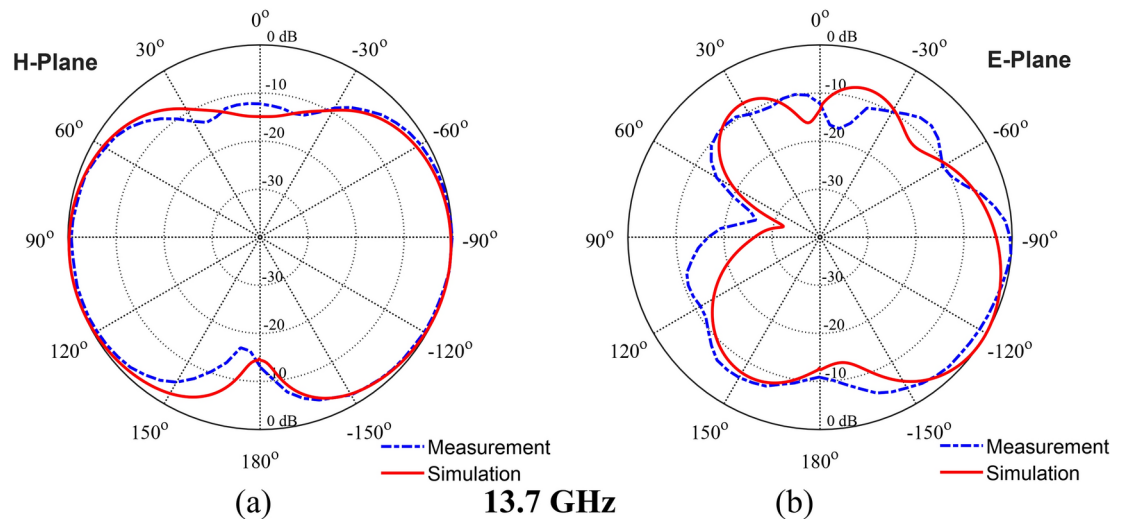
Fig. 15. Radiation pattern in ON Mode at 13.7 GHz: (a) H-plane, and (b) E-plane.
