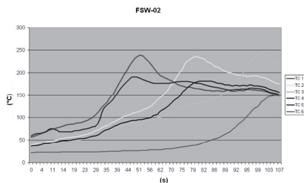
Fig. 2. Temperatures acquired in the weld FSW-02
