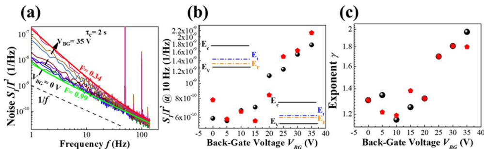
FIG. 3. (a) Normalized noise power spectra of CNNs back-gated transistor at different back-gate voltages V_{BG} . Smooth lines show the result of the fitting using Eq. (1) for two values of V_{BG} (0 V, 35 V). (b) Normalized noise power spectral density S_I/I^2 at frequency f = 10 \text{ Hz} for the same specimen vs V_{BG} . Insets show the qualitative band diagrams with relative positions of the Fermi level E_F and trap level E_t , responsible for GR noise at different V_{BG} . (c) The dependence of exponent \gamma on V_{BG} . Different symbols correspond to two consecutive measurements with a time interval of 5 min.
