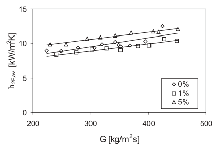
Figure 20. Average heat transfer coefficient versus mass flux density for R134a in micro-fin tube.
