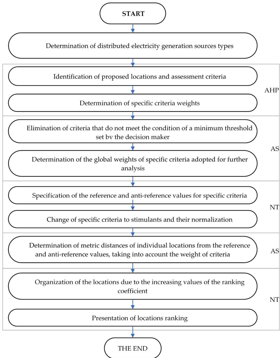
Figure 1. Method flowchart.
