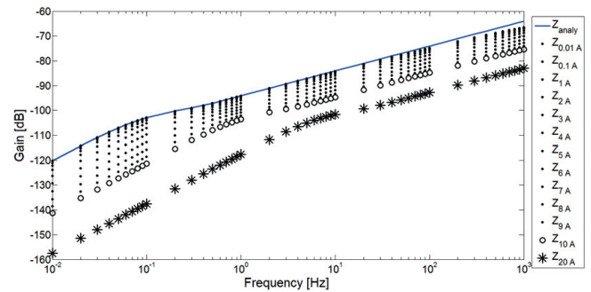
Fig. 4. Ferromagnetic sheet impedance for different saturation levels
