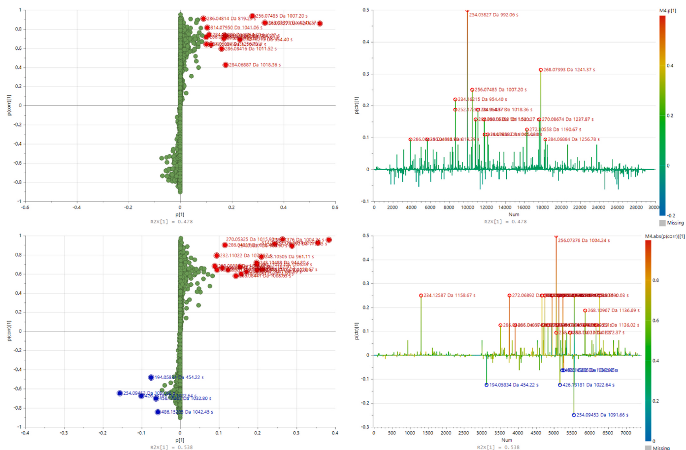
Fig. 4. Orthogonal Partial Least Squares - Discriminant Analysis (OPLS-DA) S-plots and S-lines based on LC-MS fingerprints recorded in ESI+ (top) and ESI- (bottom) for 34 propolis samples characterized by different anticandidal activity. Selected variables are marked as pairs of retention time and exact mass and highlighted in red or blue as potential markers related with high or low anticandidal activity, respectively. (For interpretation of the references to color in this figure legend, the reader is referred to the Web version of this article.)
