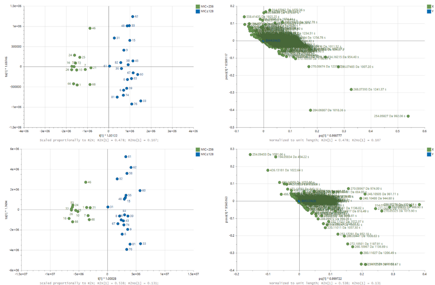
Fig. 3. Orthogonal Partial Least Squares - Discriminant Analysis (OPLS-DA) scores and loading plots (centered) based on LC-MS fingerprints recorded in ESI+ (top) and ESI- (bottom) for 34 propolis samples characterized by different anticandidal ( C. albicans ATCC 10231) activity. MIC values \leq 128 and > 256 are marked in blue and green, respectively. Numbers correspond to specific samples and variables are marked as pairs of retention time and exact mass. (For interpretation of the references to color in this figure legend, the reader is referred to the Web version of this article.)
