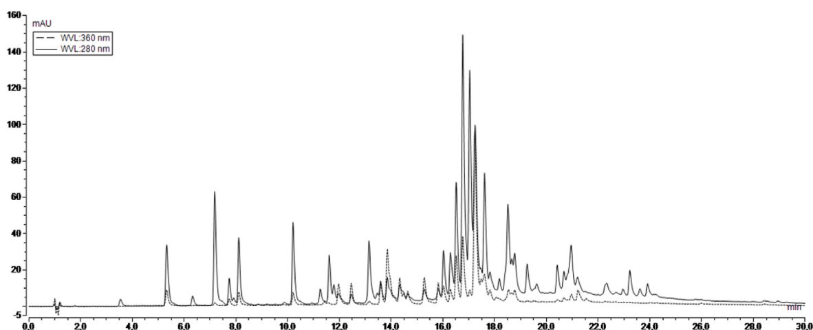
Fig. 5. Representative UHPLC chromatogram of propolis extract recorded at 280 and 360 nm.
